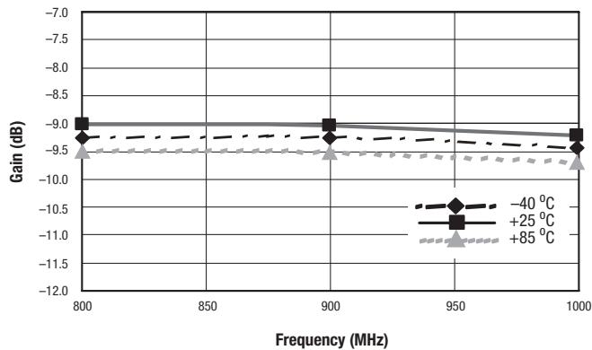
Figure 4. Power Conversion Gain vs Frequency and Temperature @ 900 MHz
