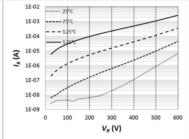
Fig. 18 Reverse Characteristics
