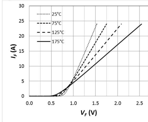
Fig. 17 Forward Characteristics
