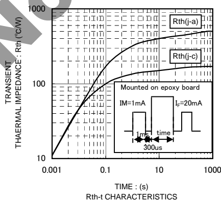
TIME : t (s) R_{th} - t CHARACTERISTICS
