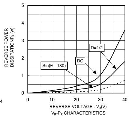
REVERSE VOLTAGE : V_R (V) V_R - P_R CHARACTERISTICS
