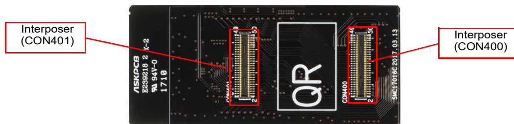
Figure 3. ARTIK 055s Interposer Board Connectors
