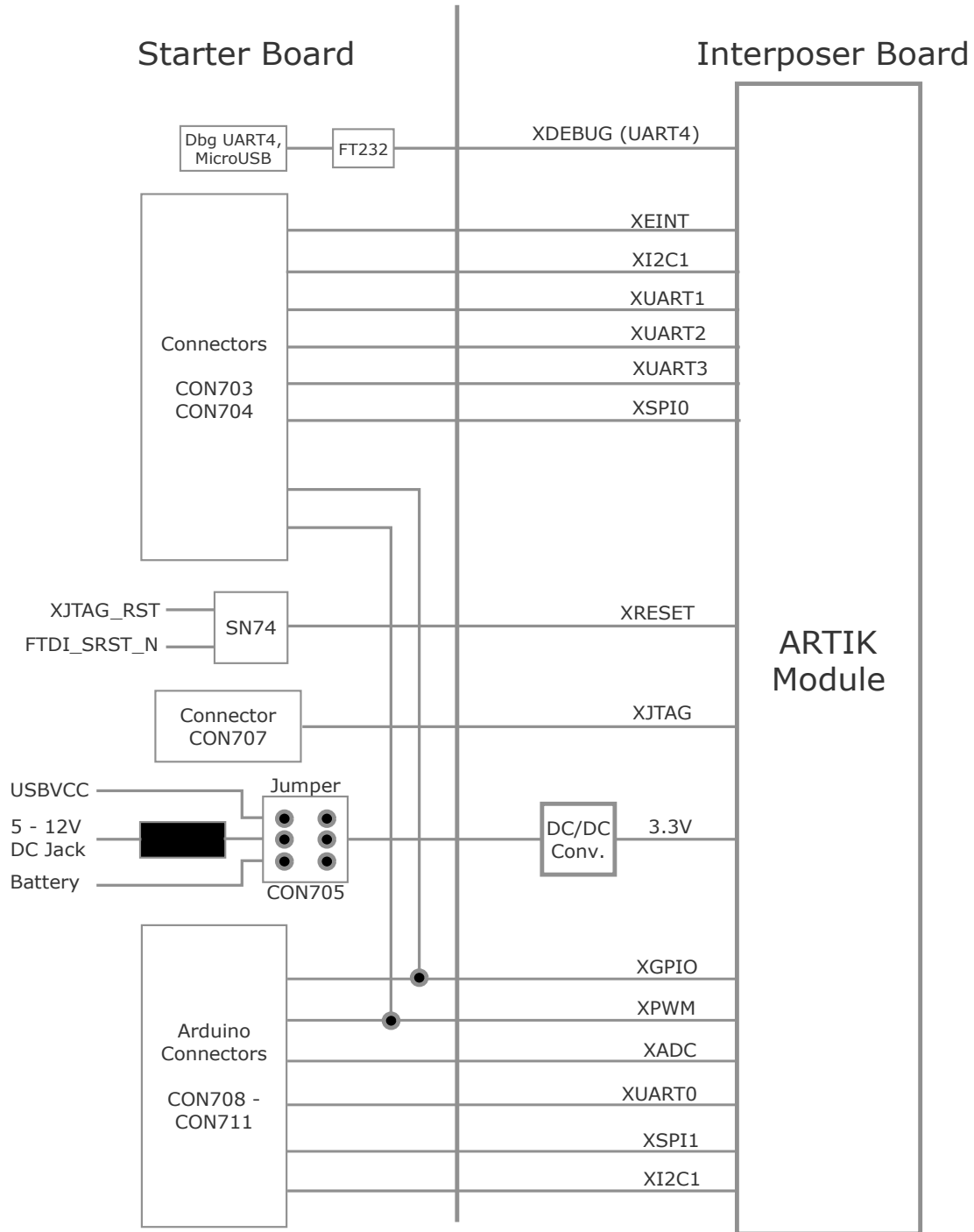
Figure 2. ARTIK 055s Development Platform System Block Diagram
