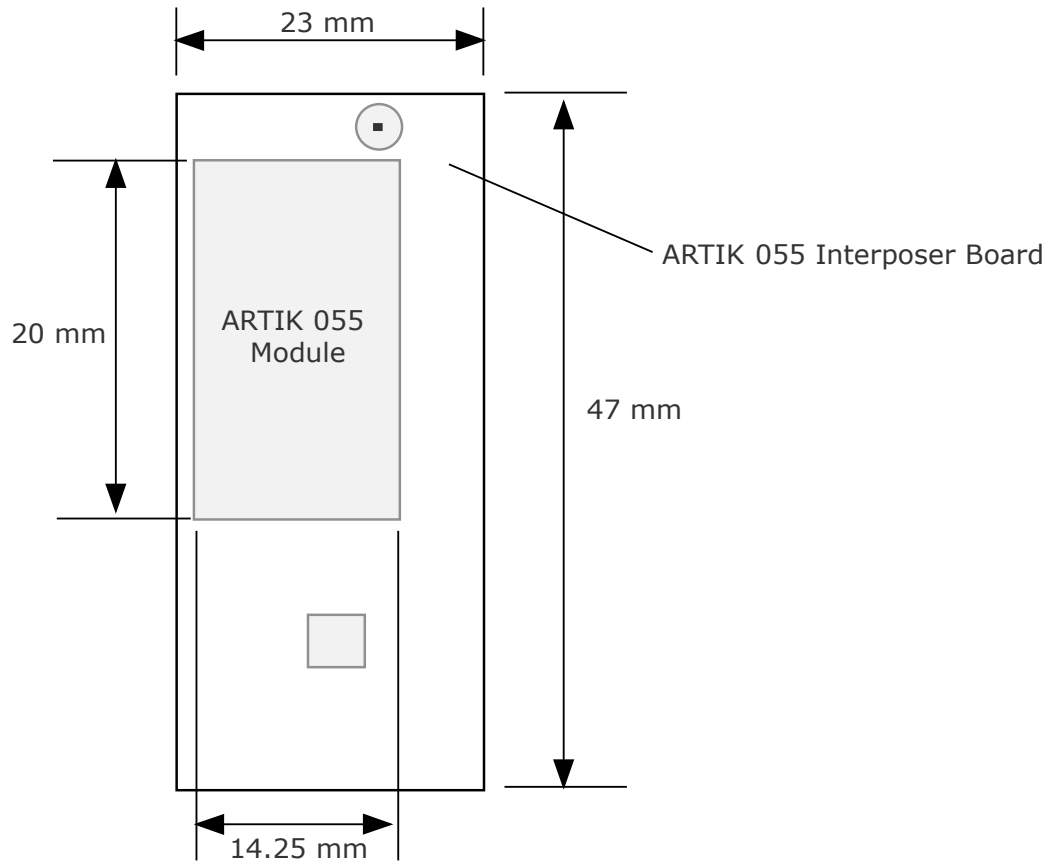
Figure 10. ARTIK 055s Interposer Board and Module Mechanical Specifications
