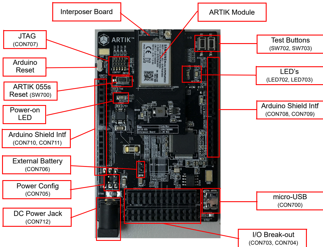
Figure 1. ARTIK 055s Development Kit Interposer and Starter Boards
