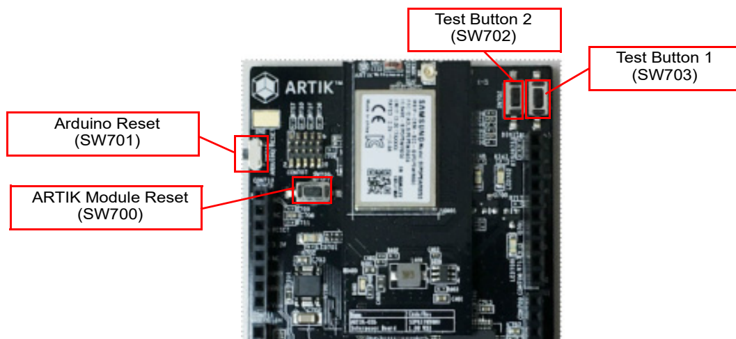
Figure 6. Location of Push Button Switches on the Starter Board
