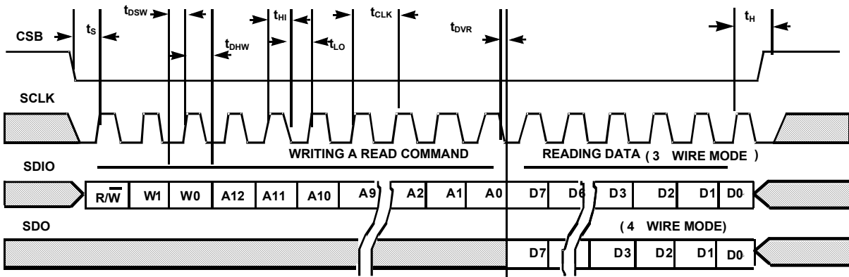
FIGURE 57. SPI READ
