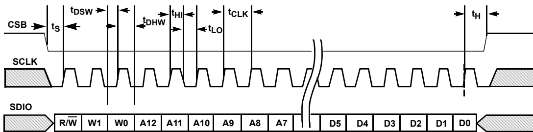
FIGURE 56. SPI WRITE
